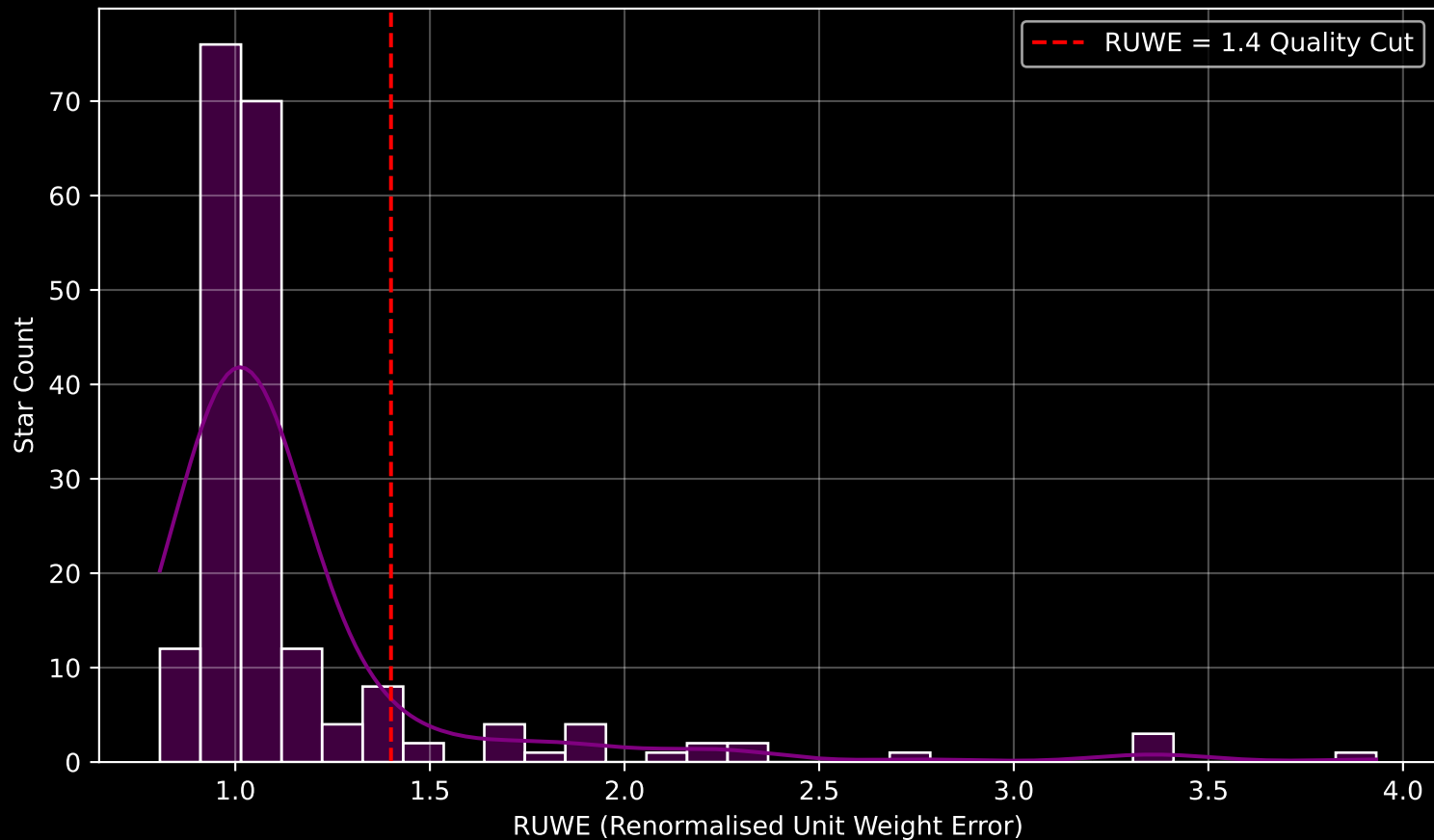
GAPOGEE DR17 Field [K2_C13_178-11_btx] RUWE Distribution (n= 203)
