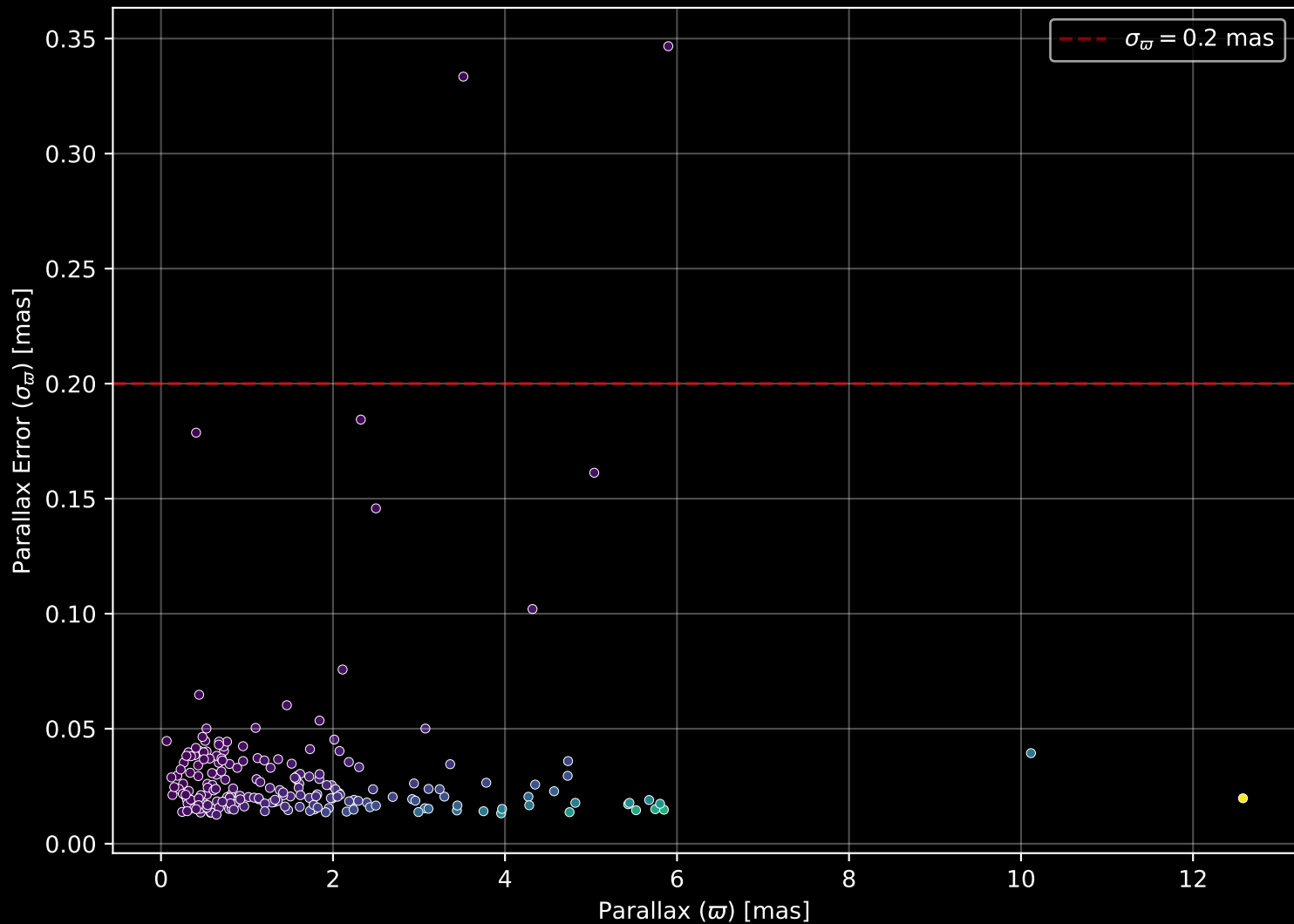
APOGEE DR17 Field: [K2_C13_178-11_btx] Parallax Quality (n= 208)
