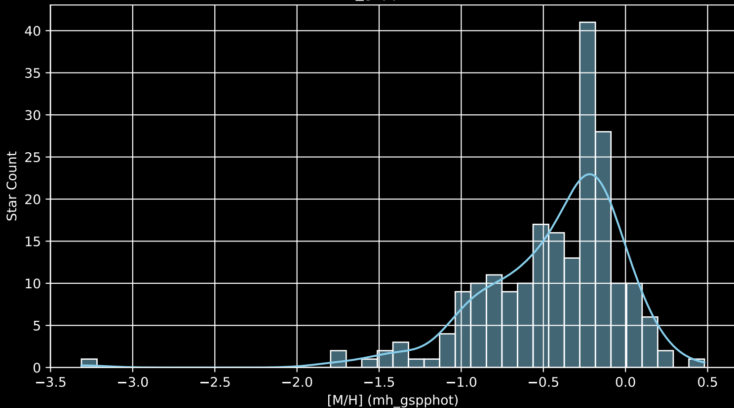
APOGEE DR17 Field: [K2_C13_178-11_btx [M/H] (mh_gspphot) (n= 208)
