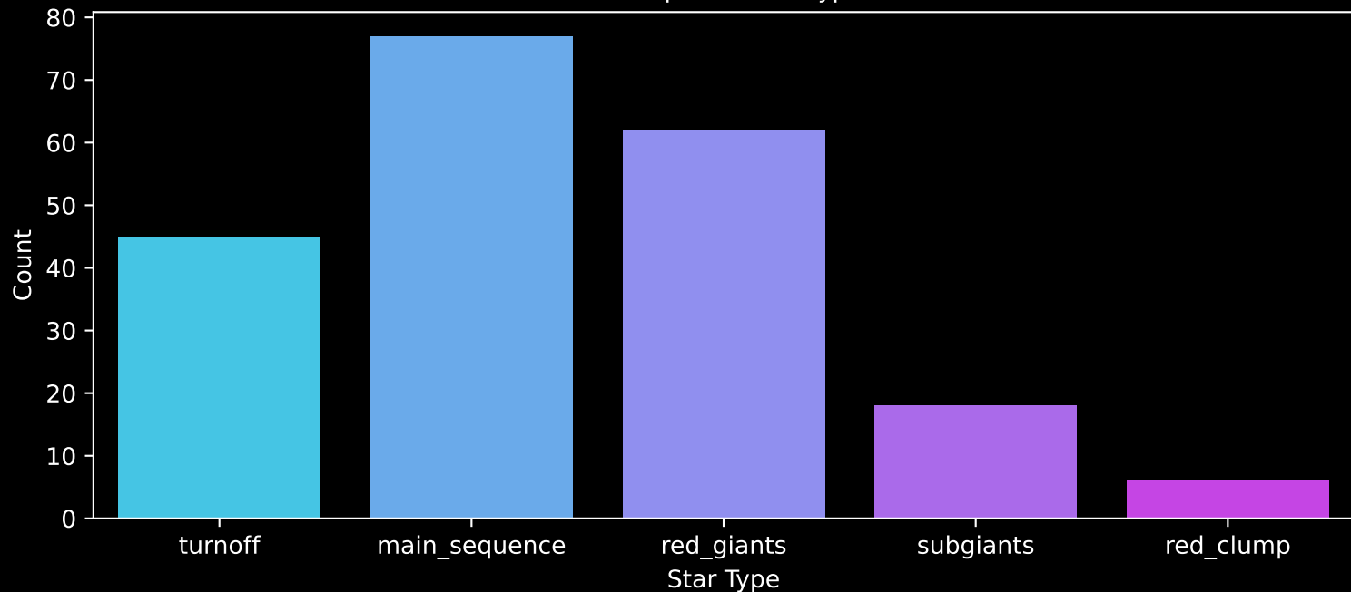
APOGEE DR17 Field: [K2_C13_178-11_btx] Count plot of Star Type
