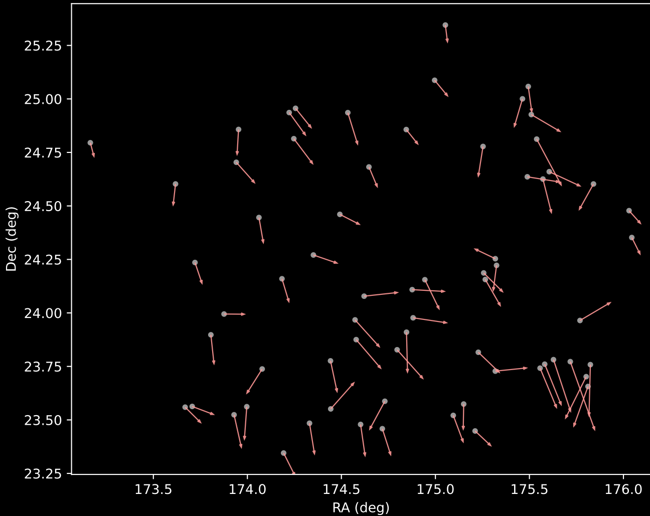
APOGEE DR17 Cluster 7 Proper Motion Vectors (n=67)
