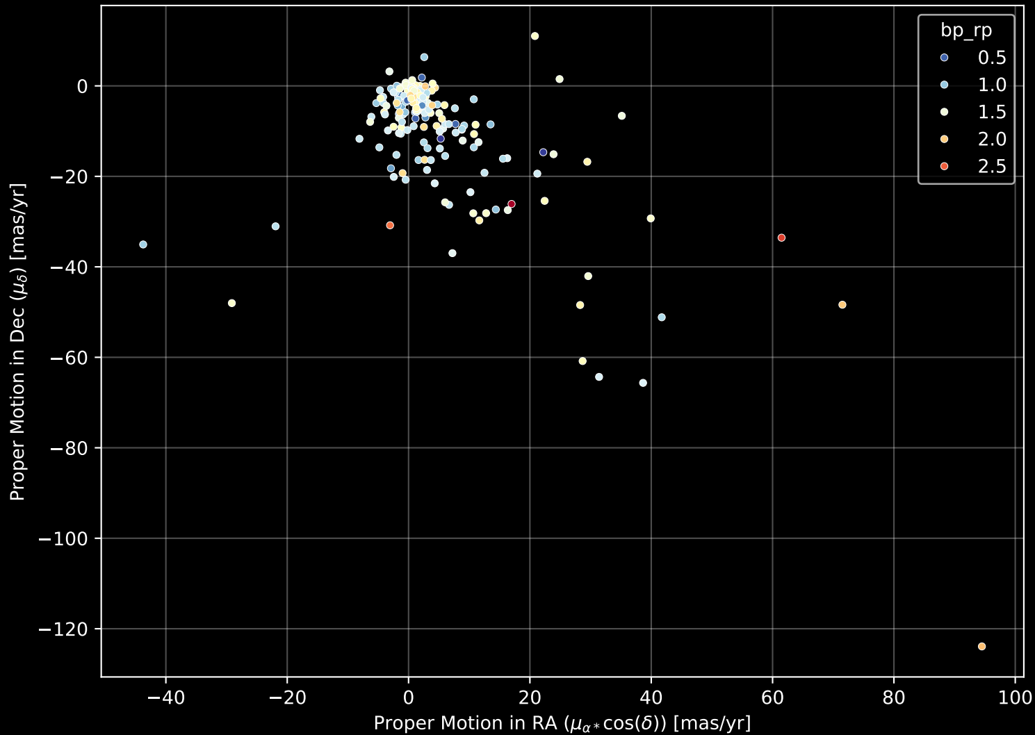
APOGEE DR17 Field: [K2_C13_178-11_btx] Proper Motion Diagram (n= 208)
