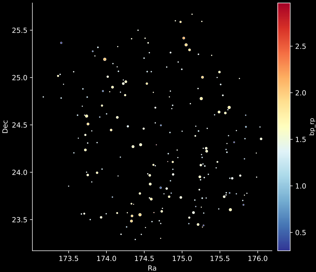
APOGEE DR17 Field: [K2_C13_178-11_btx] Stars: 208
